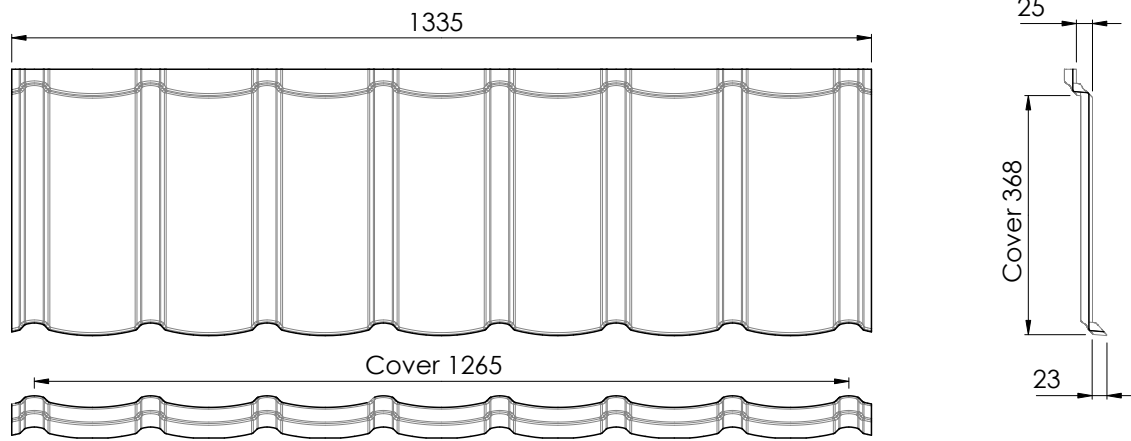
Figure 6.1 Tile Dimensions
